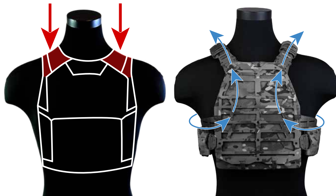
The Auto-Fit Cummerbund (Patent #: US 10605574) distributes the max loadout across/around the torso, reducing the weight on the trapezius muscles
